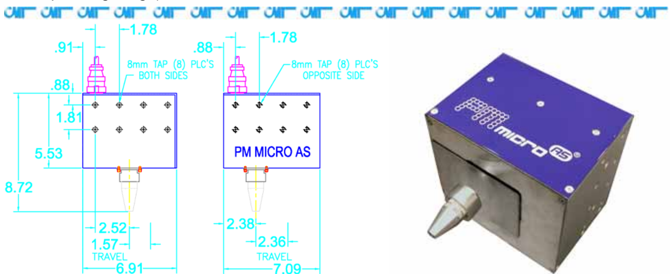
PM Micro AS shown with debris shield
