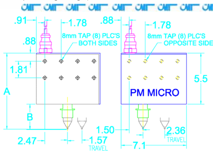
Dimensions are in inches (PM MICRO AXL drawing available upon request)
